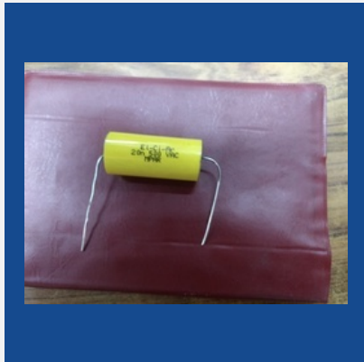
High Voltage Polypropylene Capacitors 5KV / 10KV
