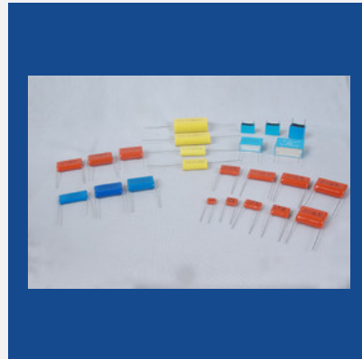
Metallized Polyester Capacitor MPT
