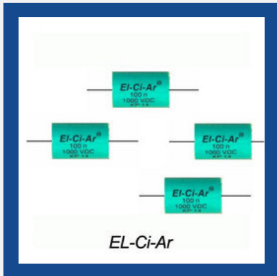
Polypropylene Axial Film Capacitor
